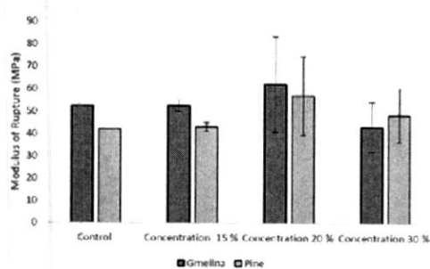
Fig. 5. MOR changes of gmelina and pine wood.
