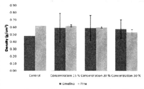
Fig. 3. Density changes of gmelina and pine wood.
